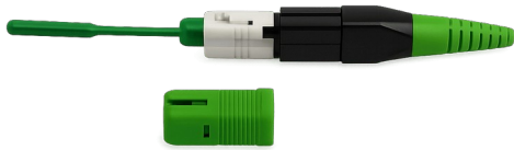
SC/APC splice-on connector and protective components.
