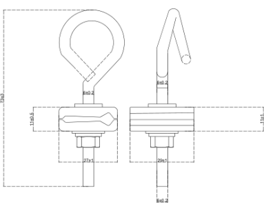
Dimension reference
